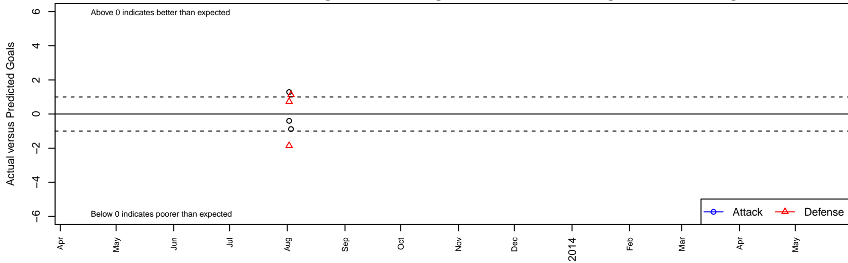
PacNW – Unk B02 Dots are actual minus expected GF (blue circles) and GA (red triangles). Blue line is smoothed change in attack strength. Red is smoothed change in defense strength.
